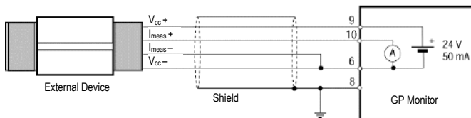
Figure 7: Installation 4 – 20 mA (4 Wires)
