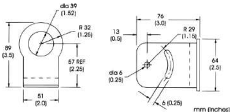
Figure 34: Fixed Mounting Bracket
