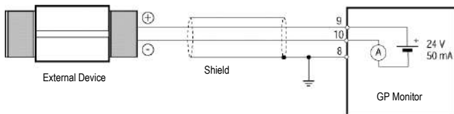
Figure 8: Installation 4 – 20 mA (2 Wires)
