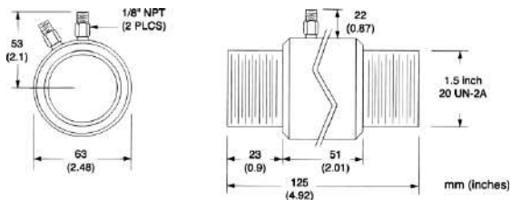
Figure 35: GPR Head with Air/Water-cooled Housing
