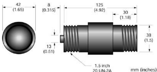
Figure 30: Dimensions for the GPR Head
