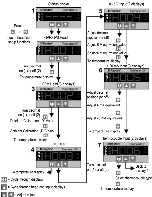
Figure 26: Head and Input Setup
