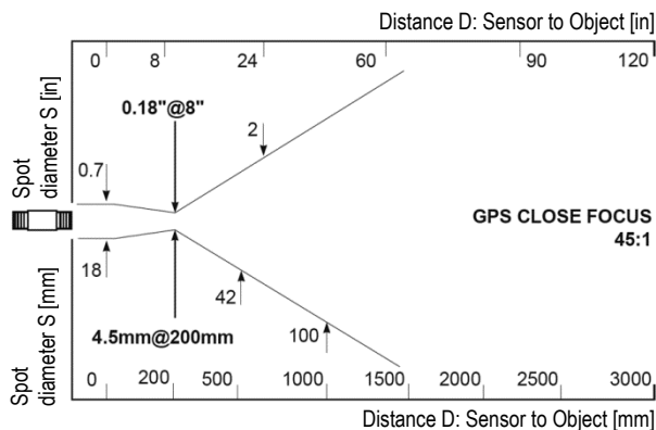
Figure 44: GPS Close Focus Optics
