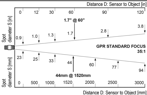
Figure 41: GPR Standard Focus Optics
