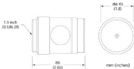
Figure 40: Sighting Viewer for GPR Head
