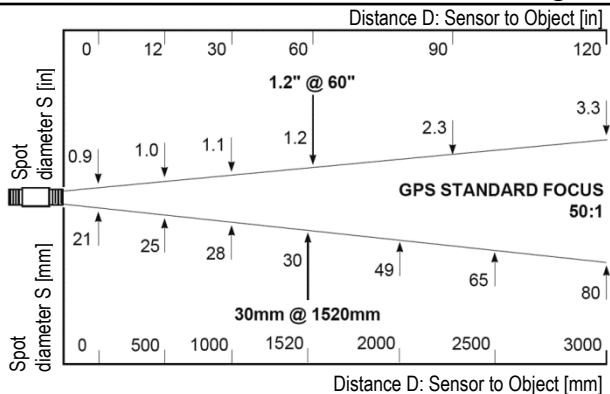
Figure 43: GPS Standard Focus Optics
