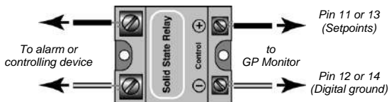
Figure 9: Relay Accessory Wiring
