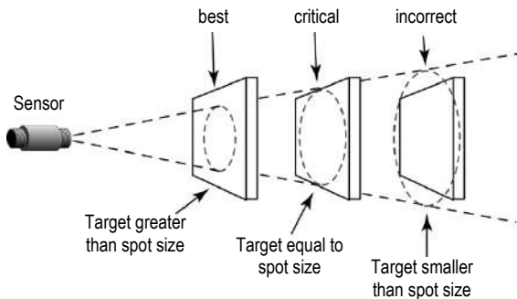
Figure 29: Proper Sensor Placement
