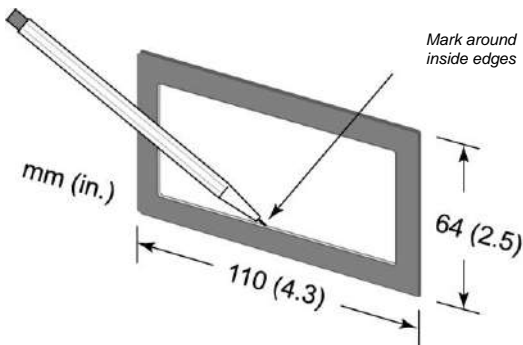
Figure 5: 1/8 DIN Cutout Template and Cosmetic Frame
