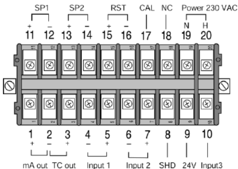
Figure 6: Terminal Block Layout
