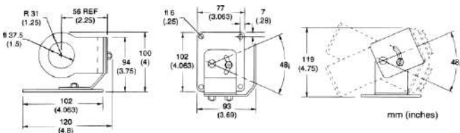
Figure 37: Adjustable Mounting Bracket
