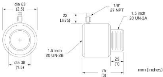
Figure 38: Air Purge Collar
