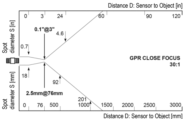
Figure 42: GPR Close Focus Optics
