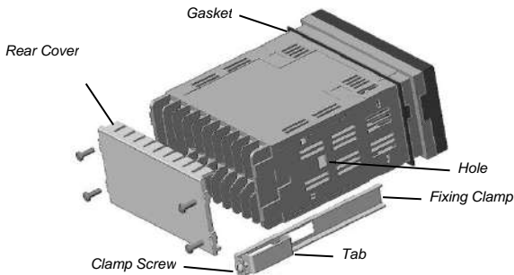
Figure 2: Mounting the Monitor
