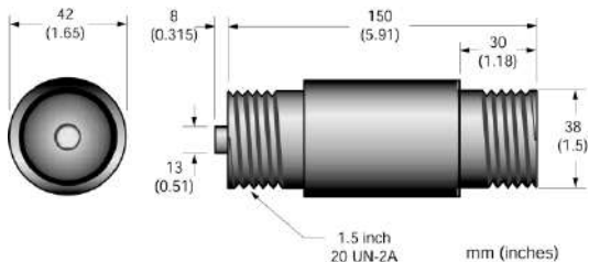
Figure 31: Dimensions for the GPS Head
